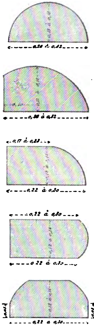
Fig. 329.—Different sections of railway-sleepers used in France. (After Boppe.)
